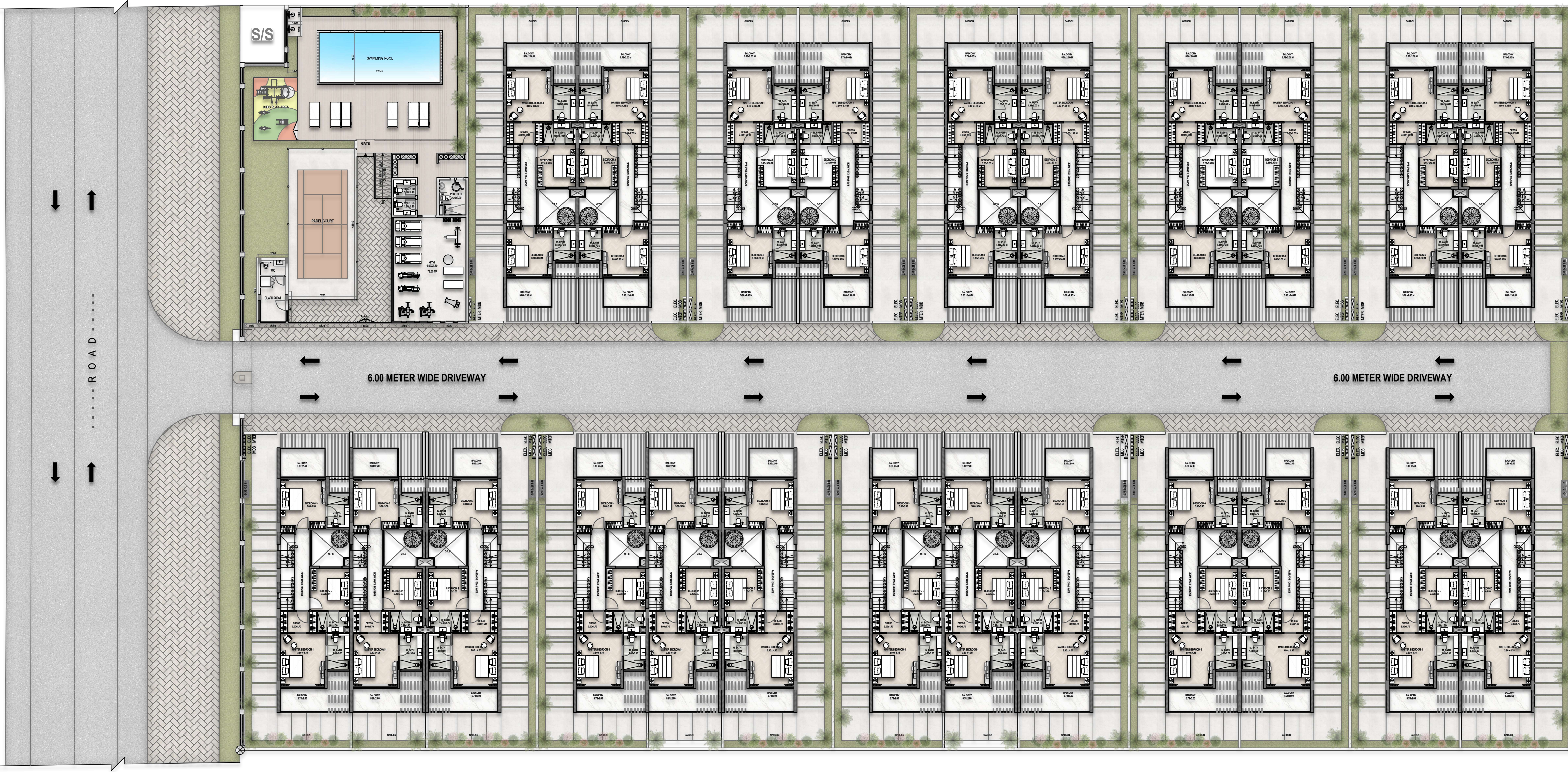
01 FIRST FLOOR MASTER PLAN SCALE 1:100@A1
